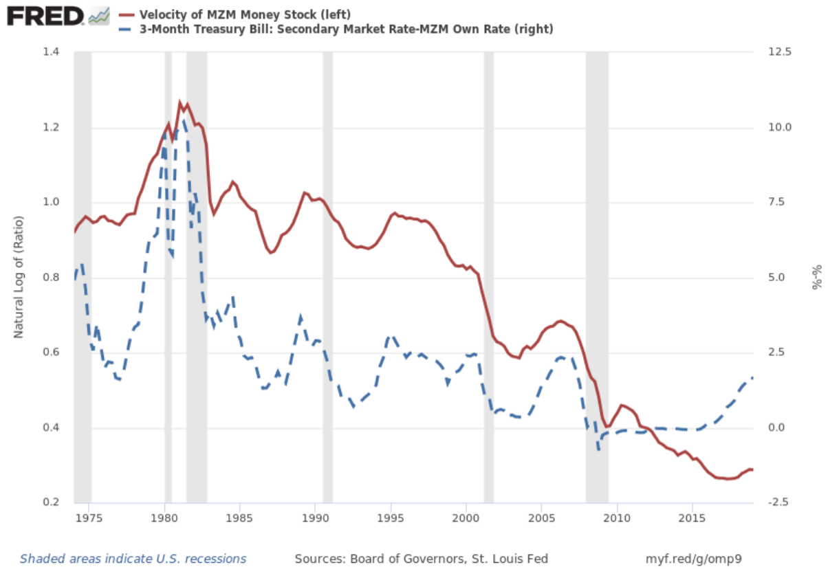
Figure 1: Velocity of MZM money stock (red) and the opportunity cost (blue dashed), 1974-2018
